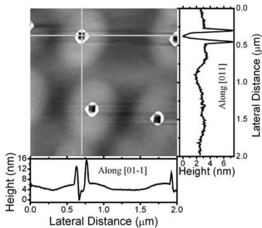
Fig. 2 AFM image of surface nanostructures formed after 1 s annealing and the corresponding height profiles
