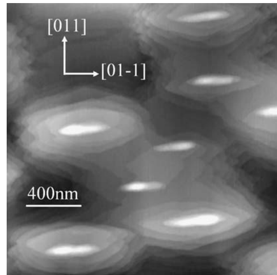
Fig. 5 AFM image of surface nanostructures formed after 10 min annealing
