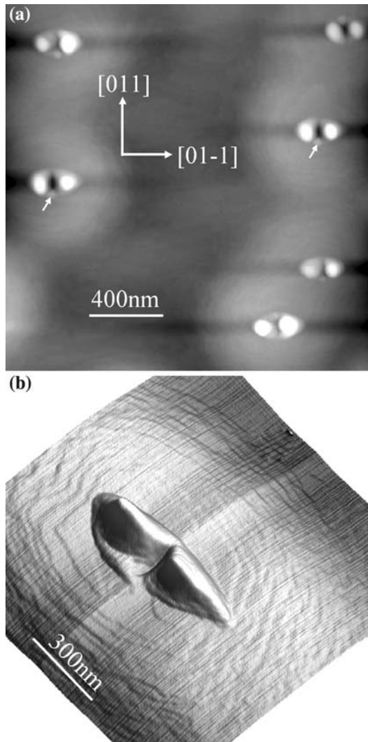
Fig. 4 (a) AFM image of QD pairs formed after 45 s annealing. (b) A single QD pair formed after 45 s annealing at 590 °C
