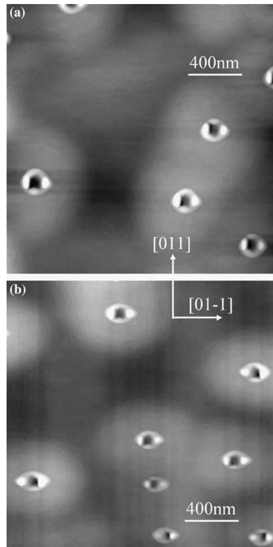
Fig. 3 (a) and (b) are AFM images of surface nanostructures formed after 5 and 15 s annealing, respectively
