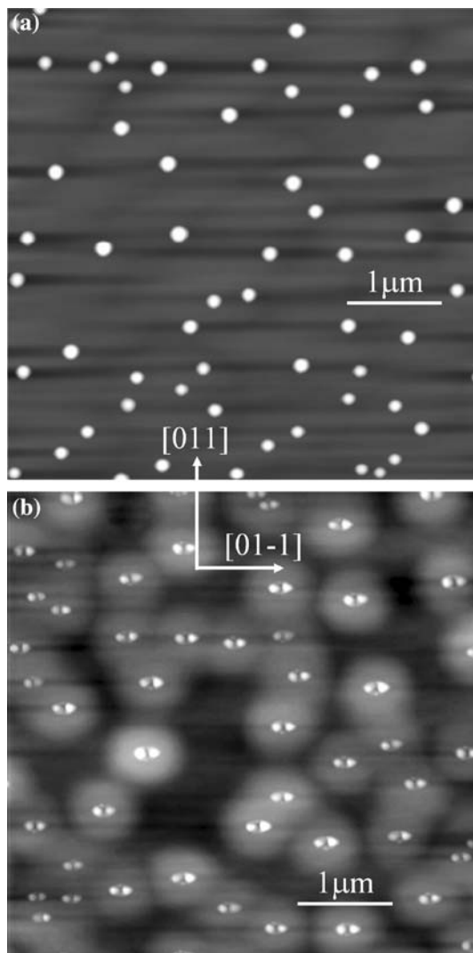
Fig. 1 (a) AFM image of Ga droplets. (b) AFM image of QD pairs formed after 45 s annealing under arsenic flux
