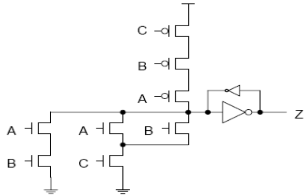
Fig. 2. Semi-Static CMOS implementation of TH23 gate Z = AB + BC + AC
