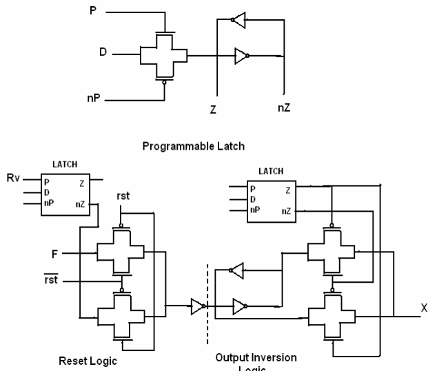
Fig. 6. Output Inversion and Reset Logic
