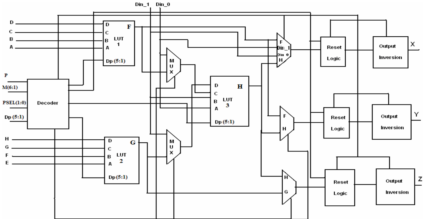
Fig. 3. Static CLB Block Diagram
