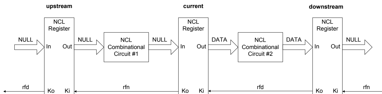
Figure 1: NCL Pipeline.
