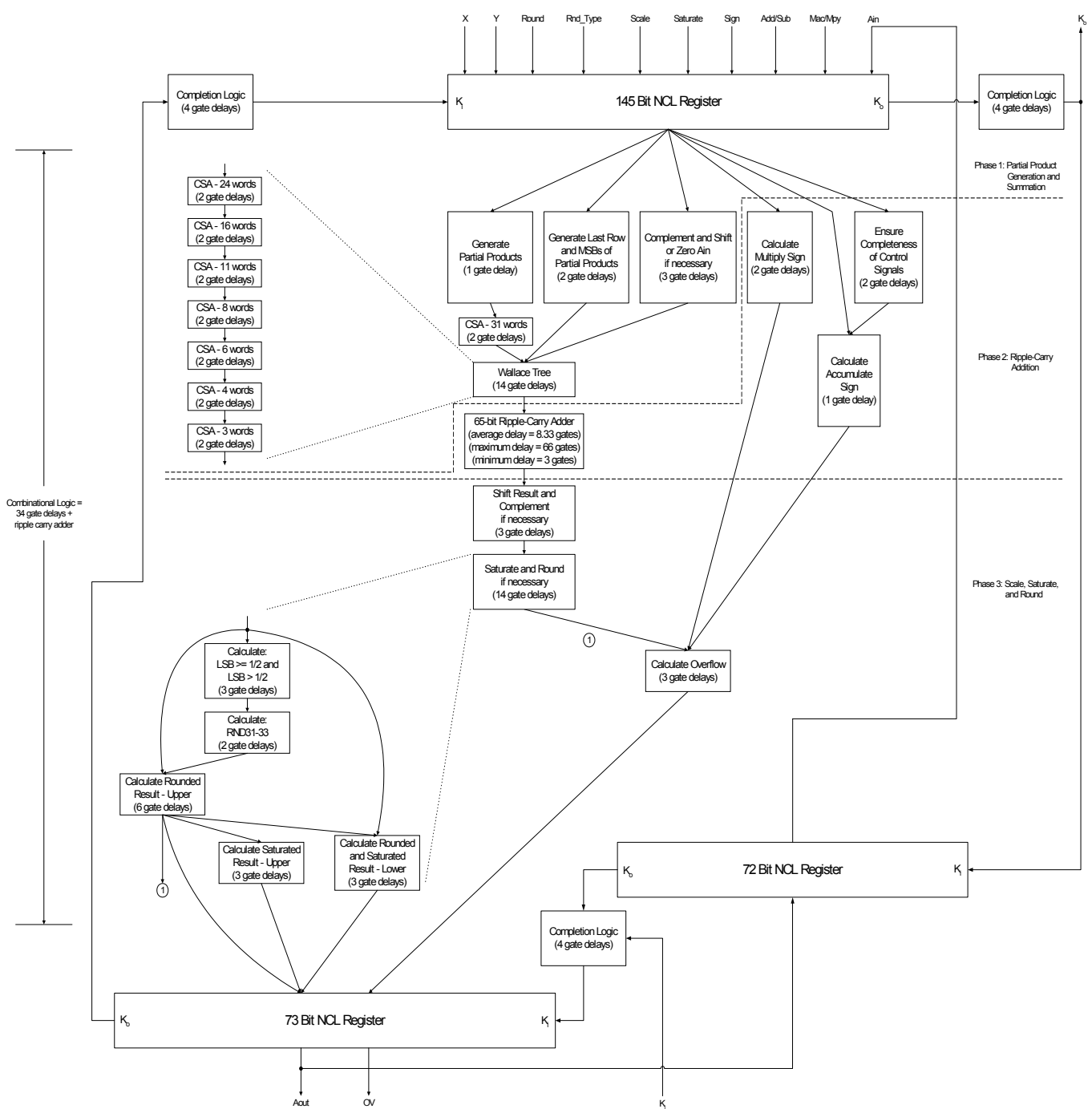
Figure 4. Non-pipelined Modified Baugh-Wooley MAC.
