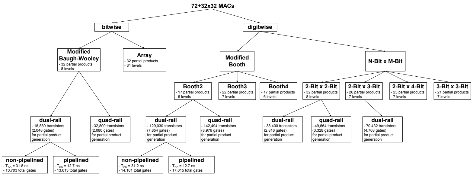
Figure 3. Taxonomy of 72+32x32 MACs.
