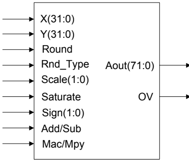
Figure 2: MAC block diagram.
