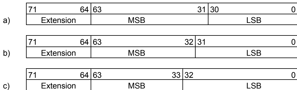
Figure 5. Partitioning of the Output for a) up-scaling, b) no scaling, and c) down-scaling.
