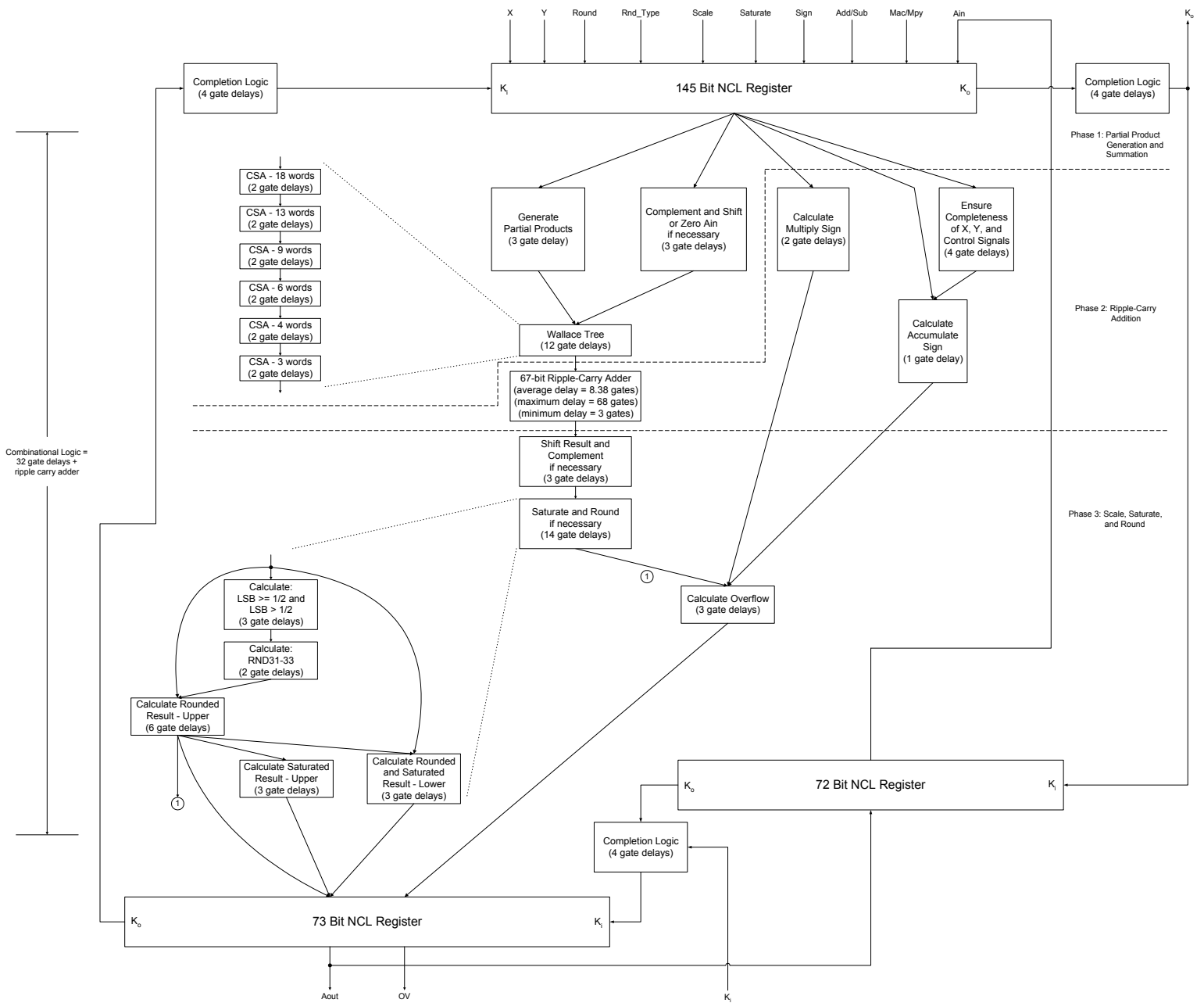
Figure 6. Non-pipelined Modified Booth2 MAC.
