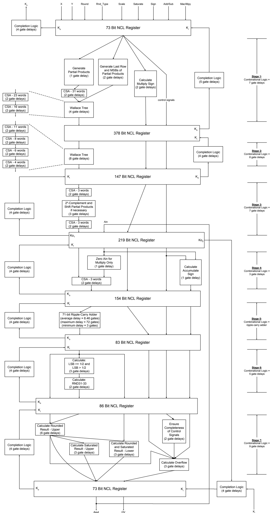
Figure 7. Pipelined Modified Baugh-Wooley MAC.
