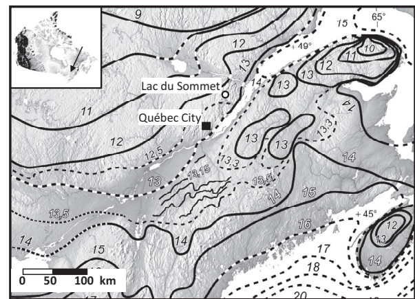
Figure 1. Location of Lac du Sommet (830 m a.s.l.; 47°43'N, 70°40'W). Digital elevation map of the study area. Solid contour lines indicate dated isochrones of ice retreat in cal. kyr BP. Dashed lines are interpolated years (Pierre Richard, unpublished data)
